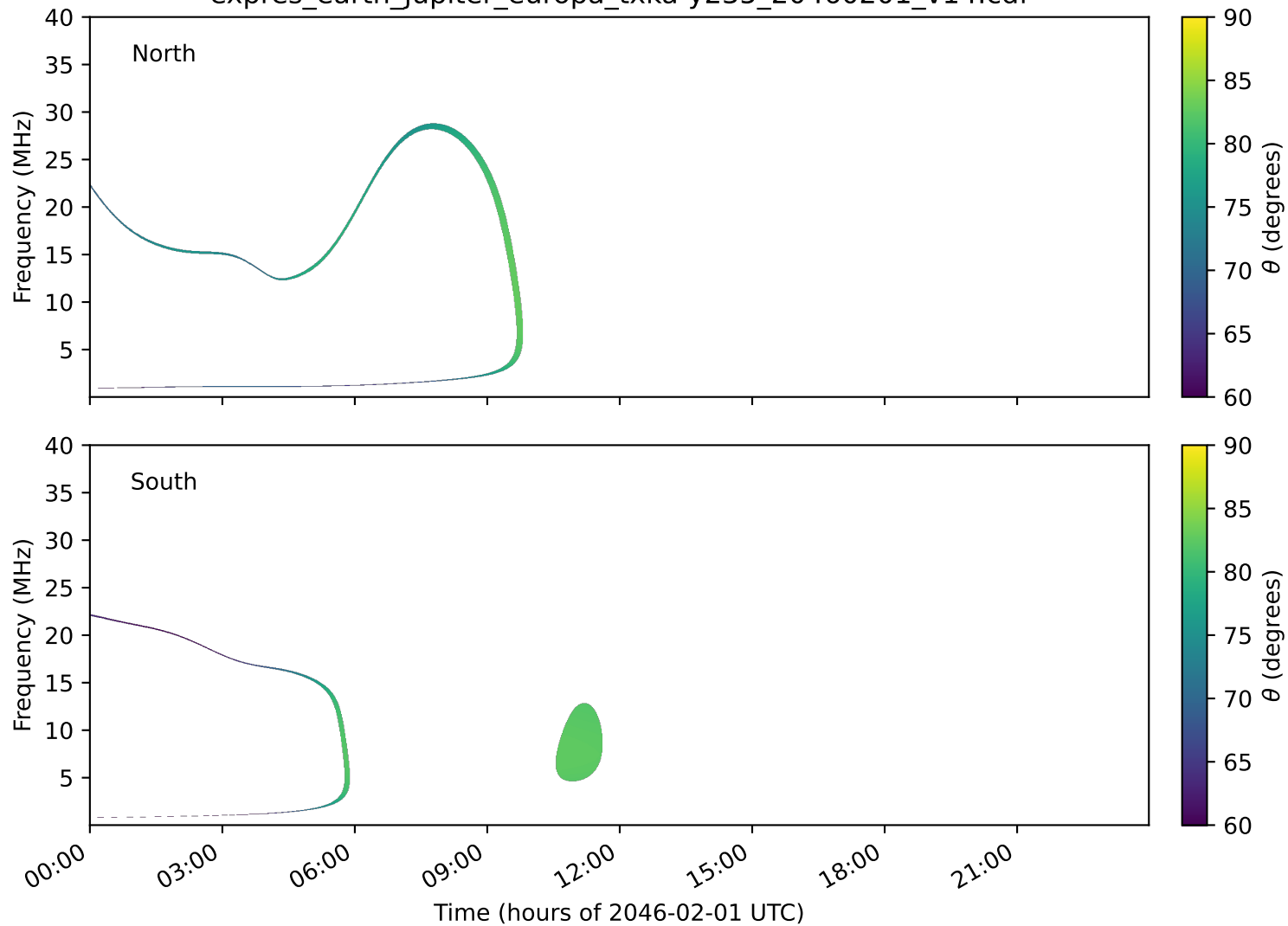
expres_earth_jupiter_europa_txka-y235_20460201_v14.cdf
