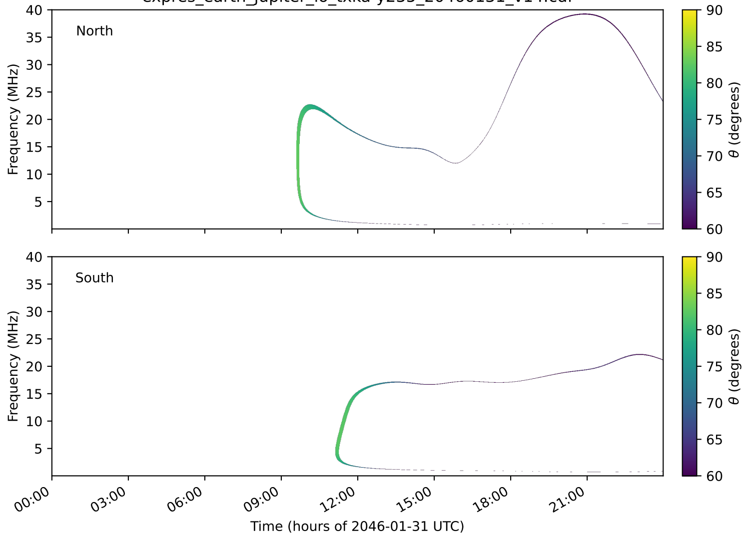
expres_earth_jupiter_io_txka-y235_20460131_v14.cdf
