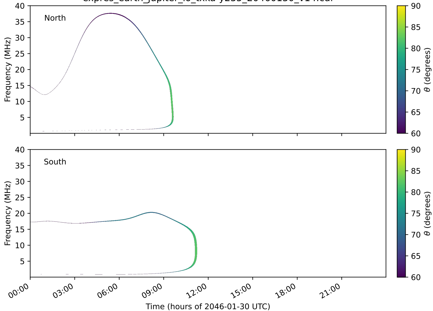
expres_earth_jupiter_io_txka-y235_20460130_v14.cdf
