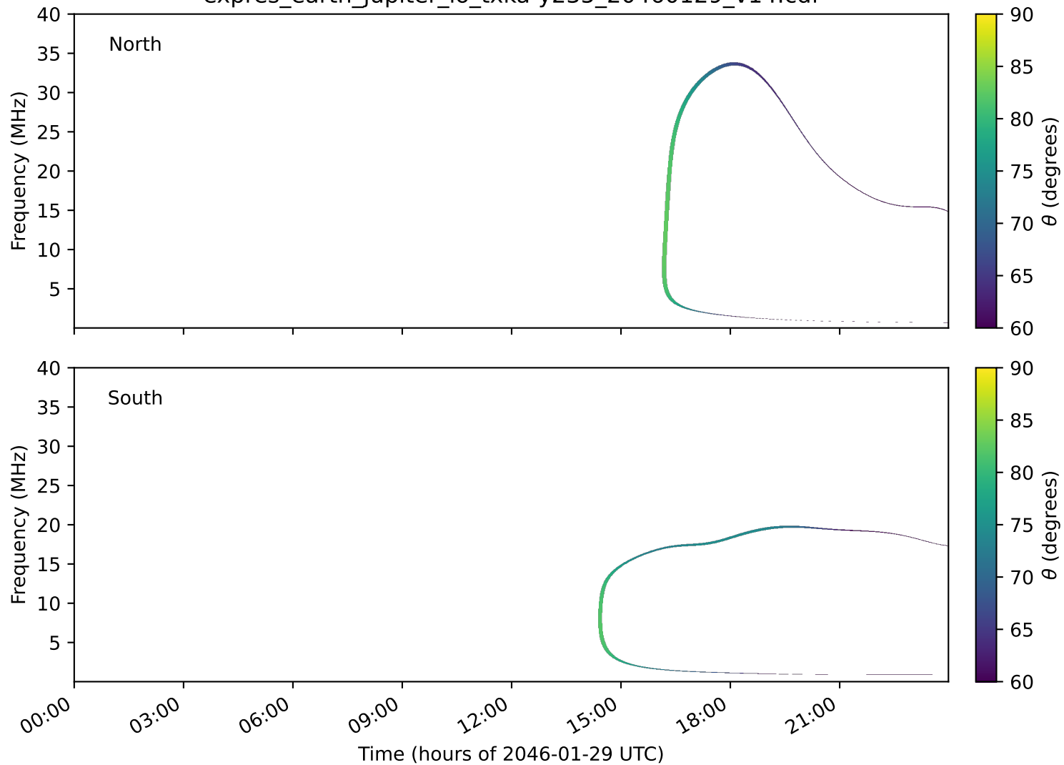
expres_earth_jupiter_io_txka-y235_20460129_v14.cdf
