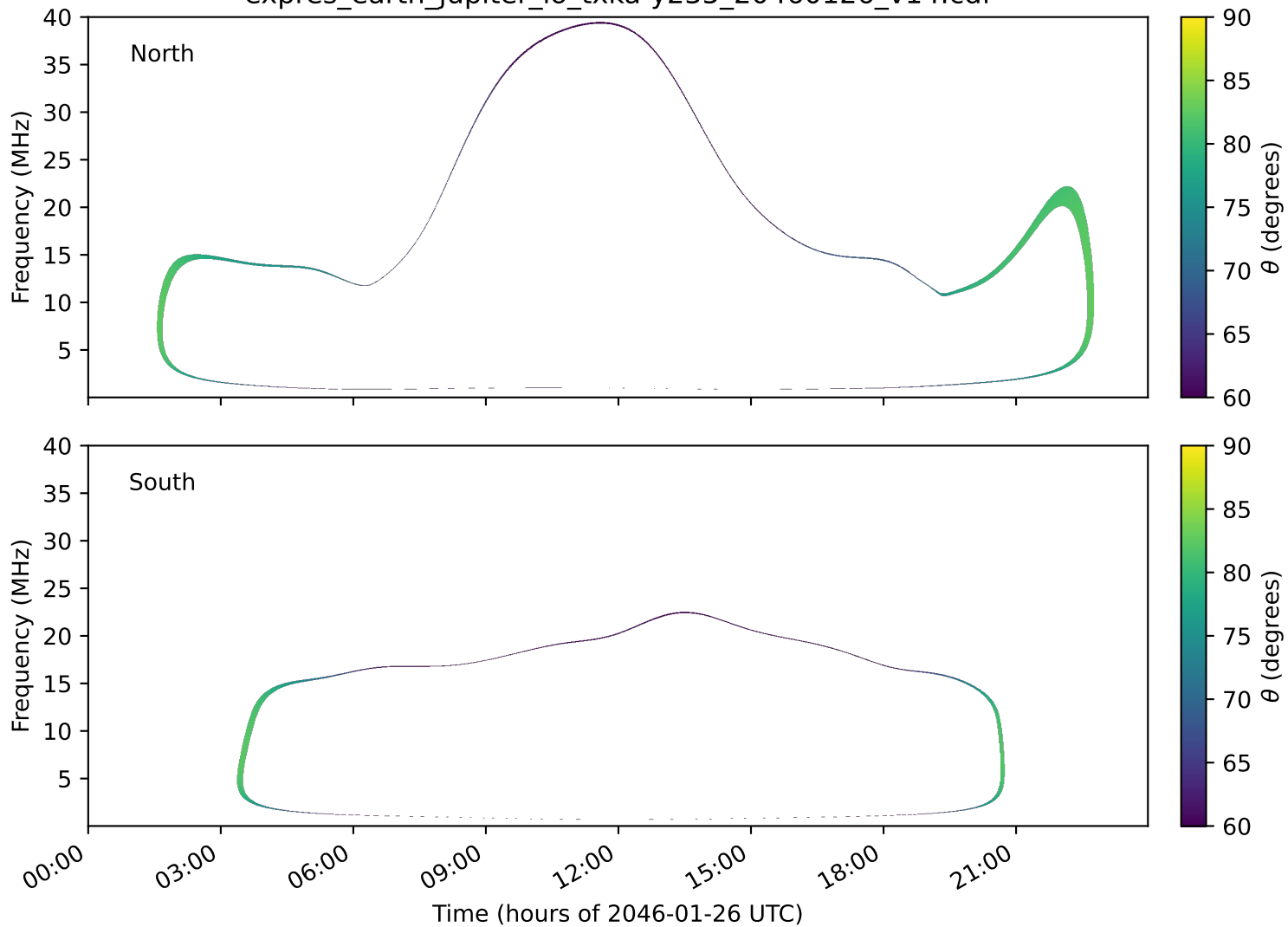
expres_earth_jupiter_io_txka-y235_20460126_v14.cdf
