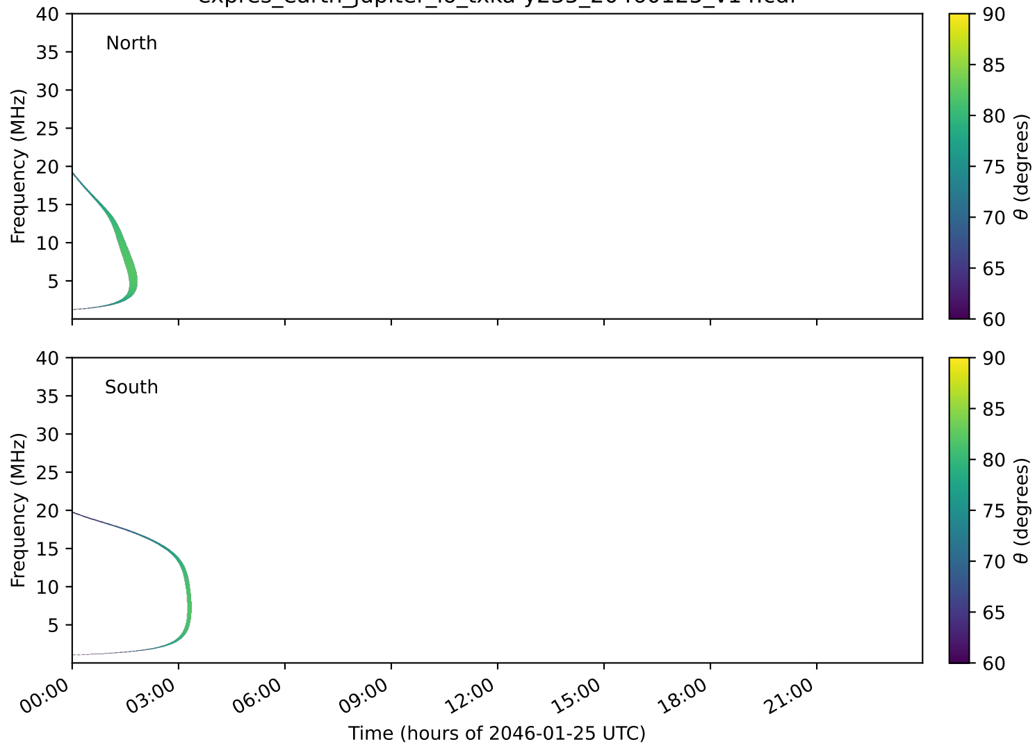
expres_earth_jupiter_io_txka-y235_20460125_v14.cdf
