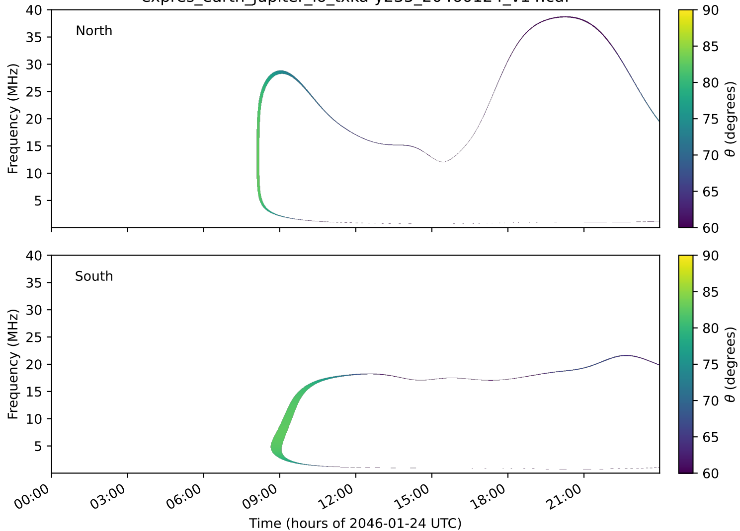
expres_earth_jupiter_io_txka-y235_20460124_v14.cdf
