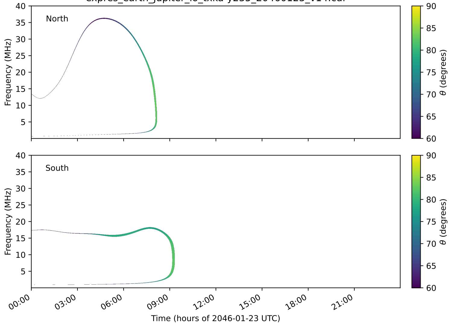
expres_earth_jupiter_io_txka-y235_20460123_v14.cdf
