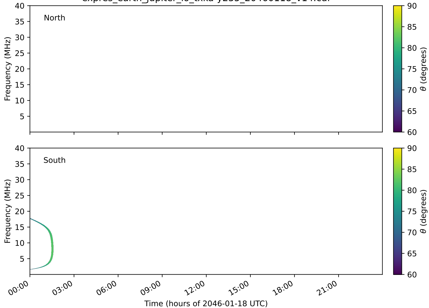
expres_earth_jupiter_io_txka-y235_20460118_v14.cdf
