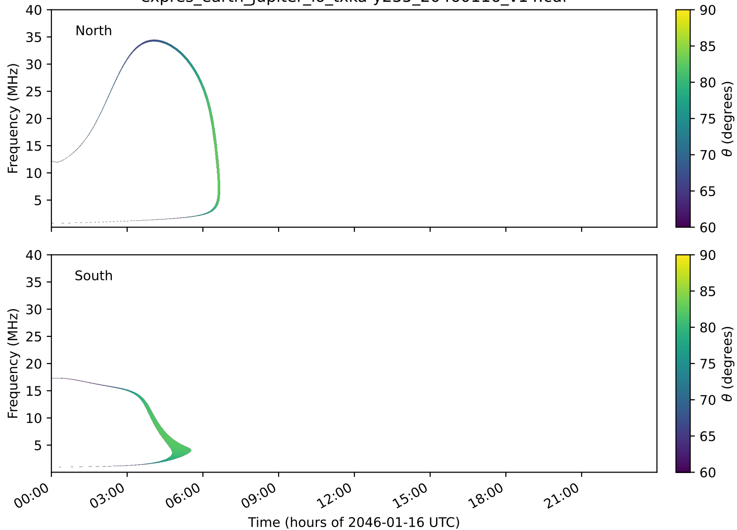
expres_earth_jupiter_io_txka-y235_20460116_v14.cdf
