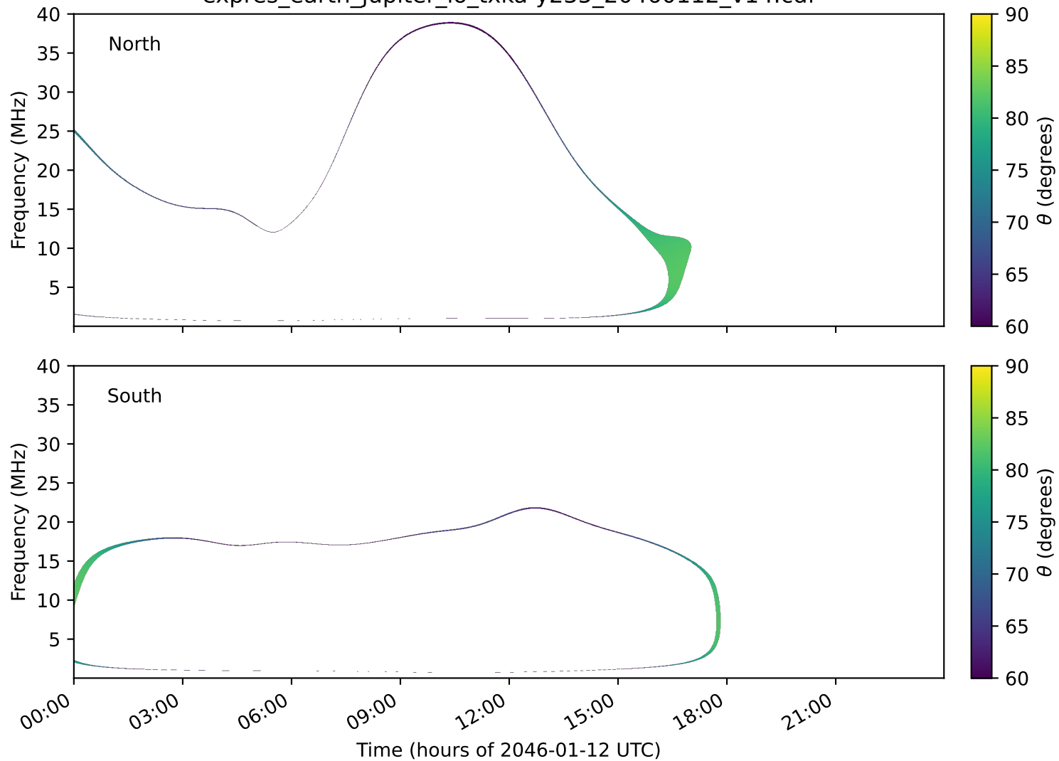
expres_earth_jupiter_io_txka-y235_20460112_v14.cdf
