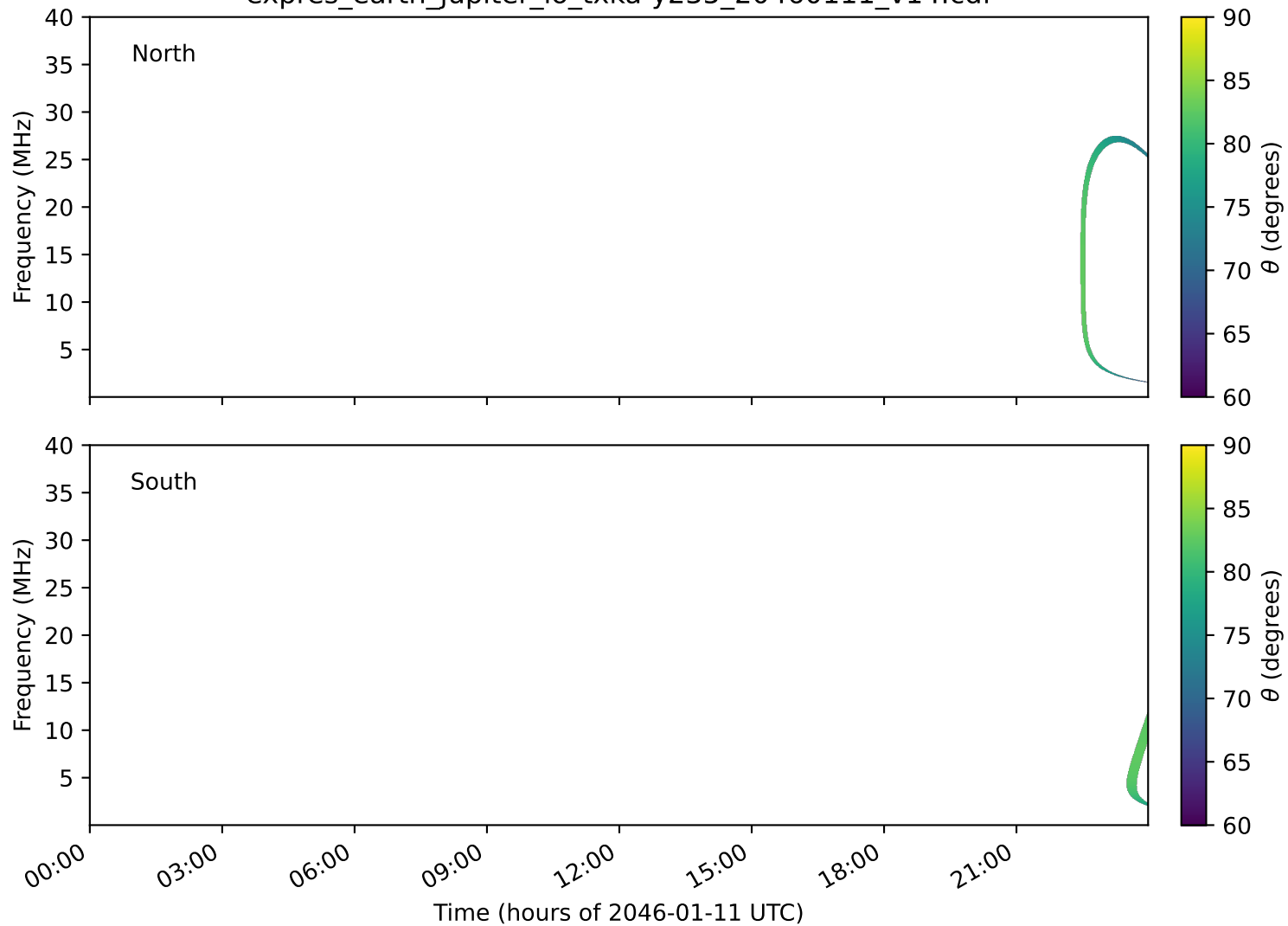
expres_earth_jupiter_io_txka-y235_20460111_v14.cdf
