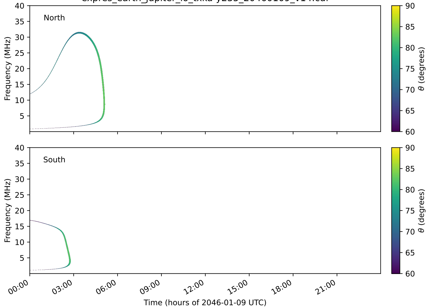
expres_earth_jupiter_io_txka-y235_20460109_v14.cdf
