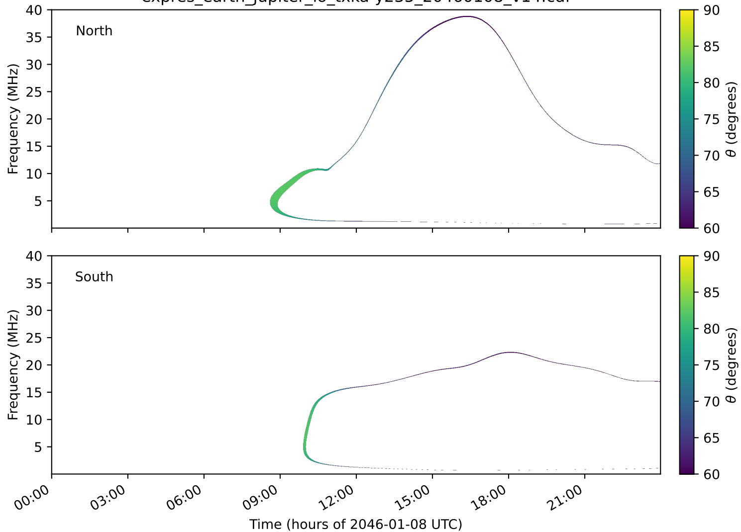
expres_earth_jupiter_io_txka-y235_20460108_v14.cdf
