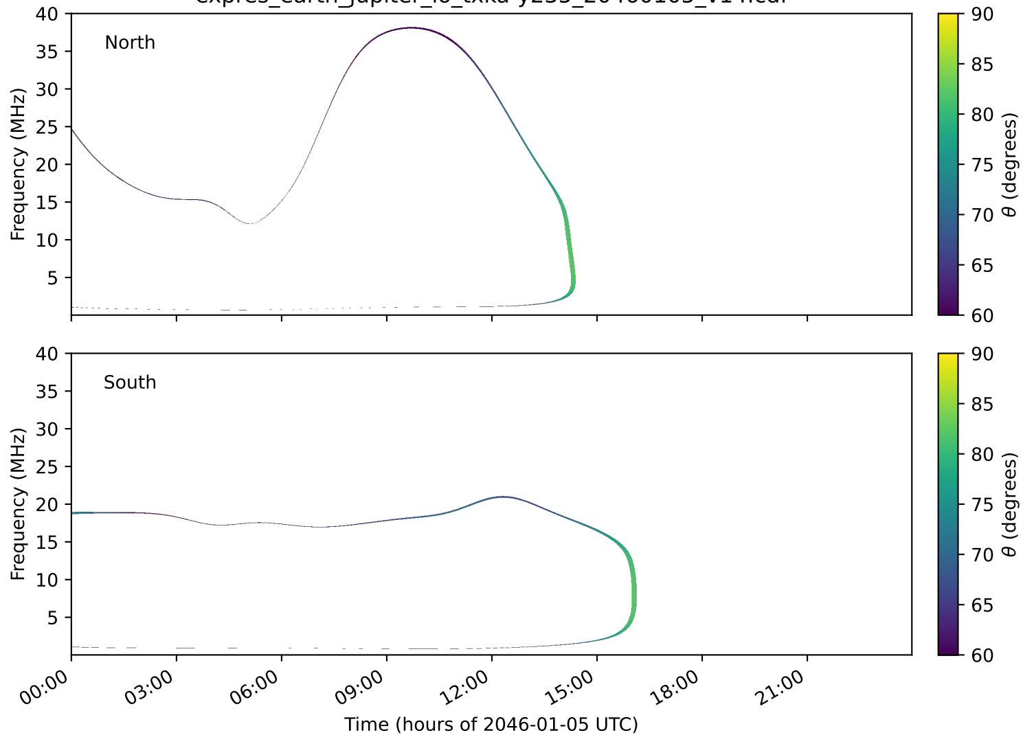
expres_earth_jupiter_io_txka-y235_20460105_v14.cdf
