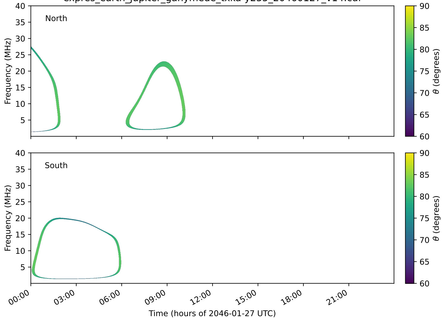
expres_earth_jupiter_ganymede_txka-y235_20460127_v14.cdf
