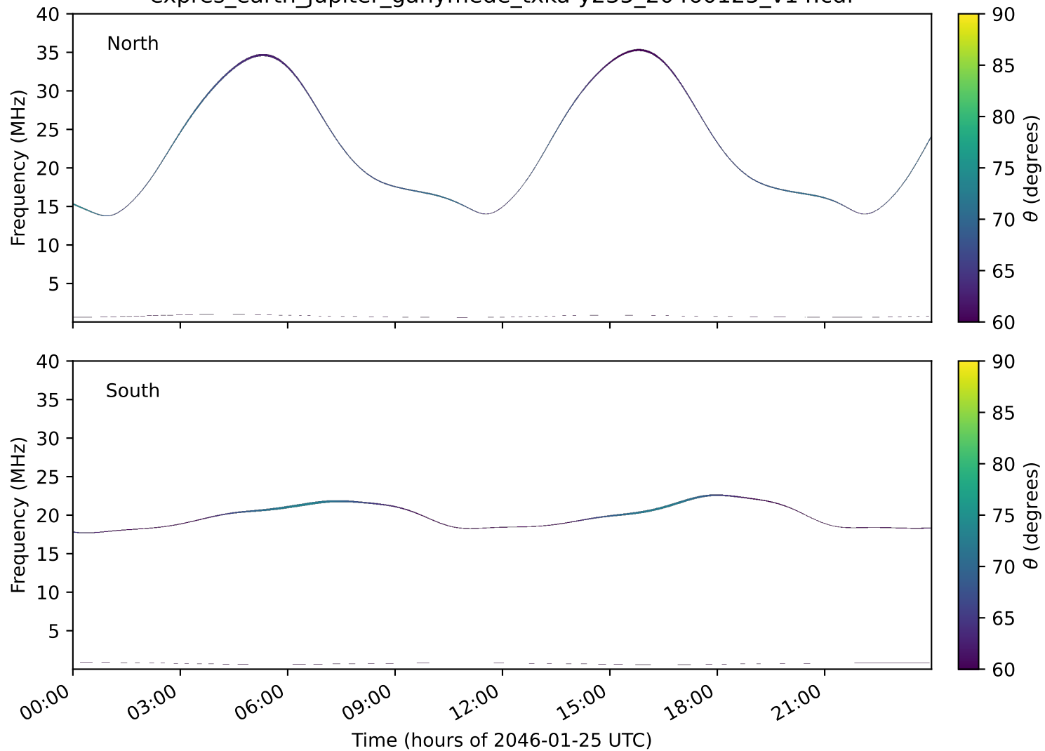
expres_earth_jupiter_ganymede_txka-y235_20460125_v14.cdf
