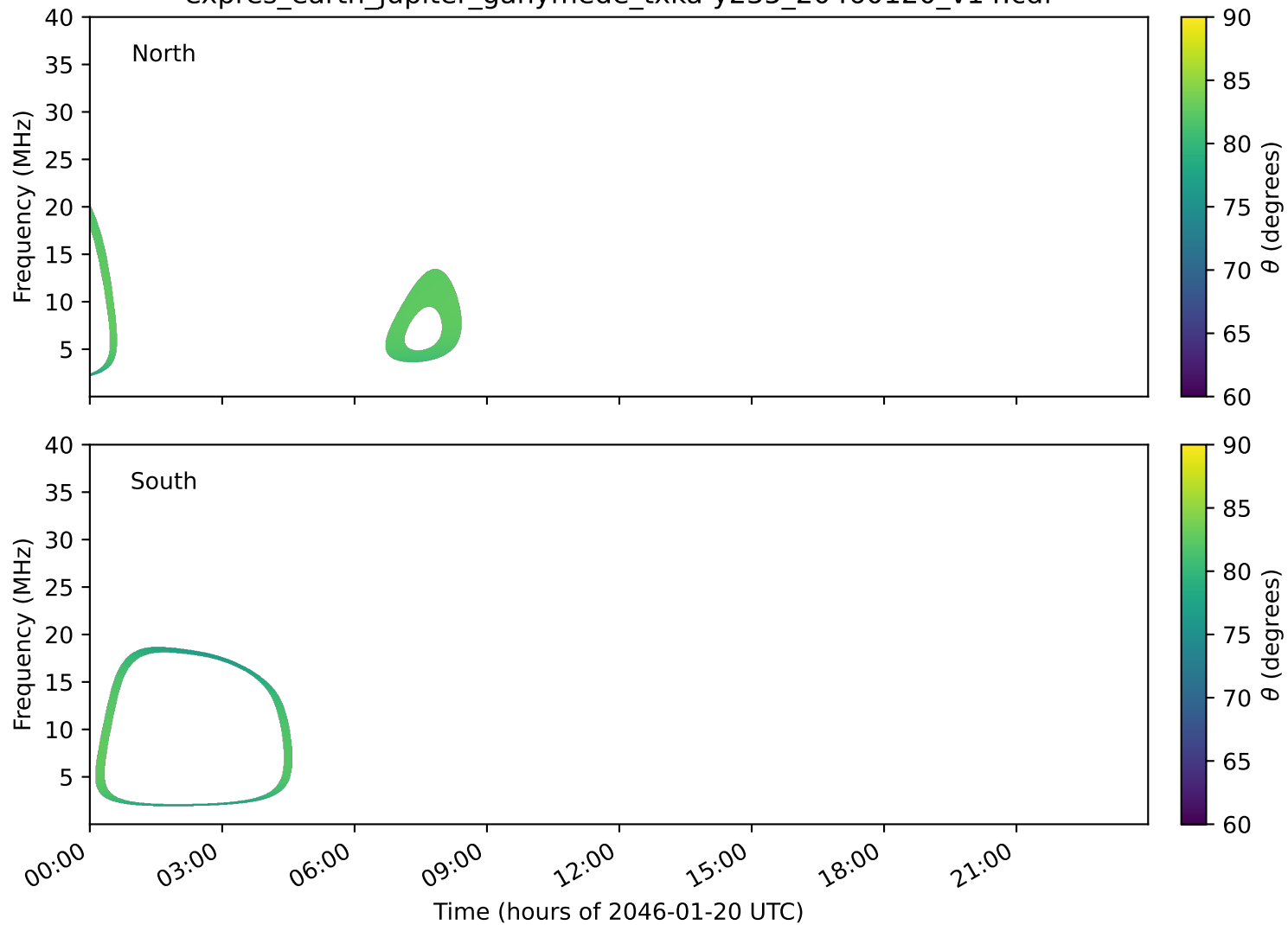
expres_earth_jupiter_ganymede_txka-y235_20460120_v14.cdf
