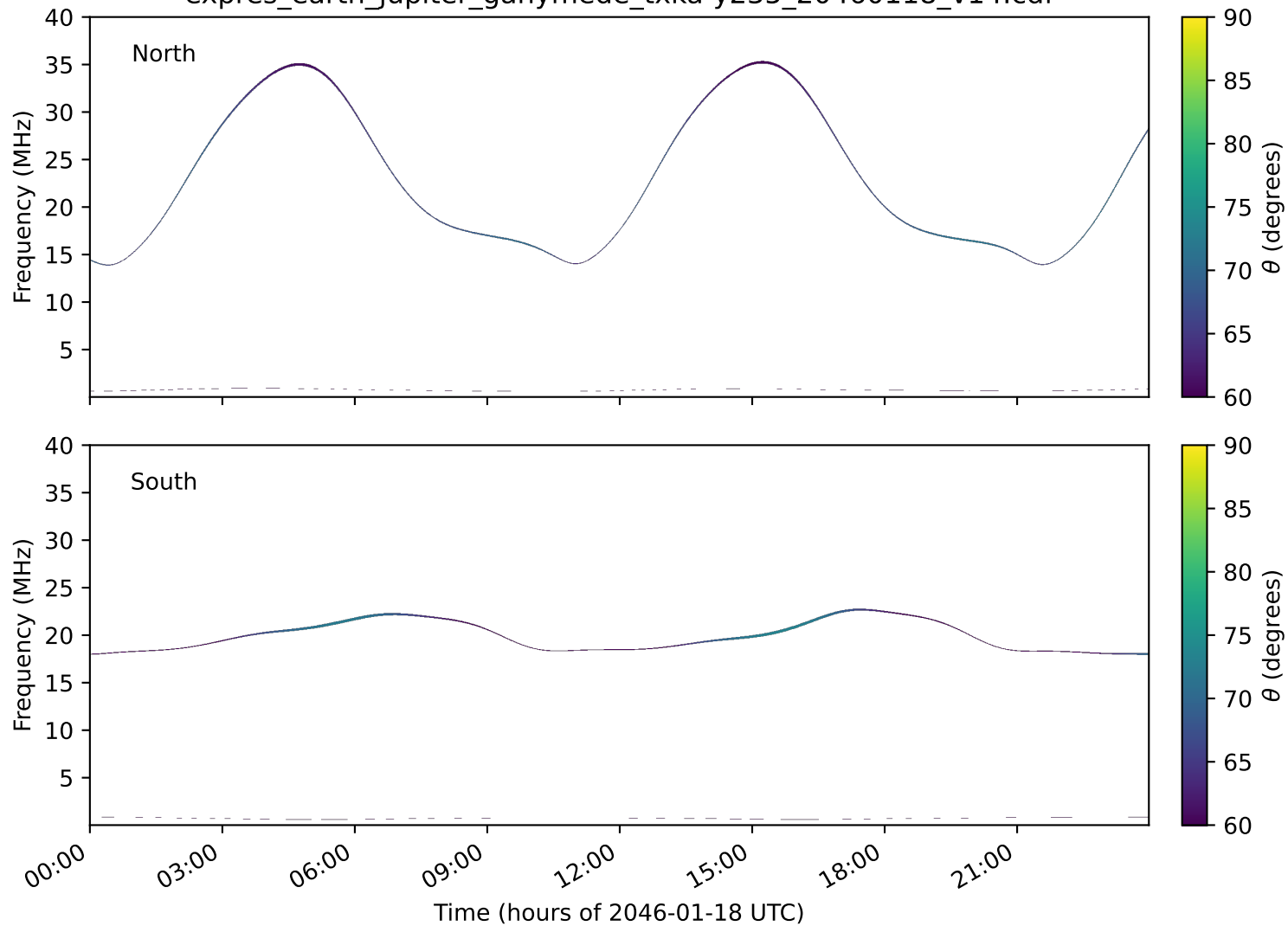
expres_earth_jupiter_ganymede_txka-y235_20460118_v14.cdf
