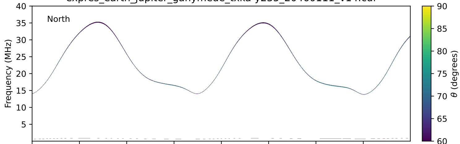
expres_earth_jupiter_ganymede_txka-y235_20460111_v14.cdf
