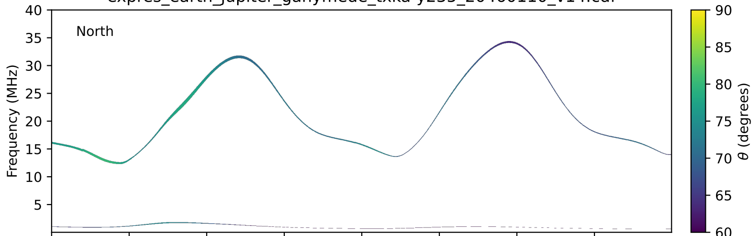
expres_earth_jupiter_ganymede_txka-y235_20460110_v14.cdf
