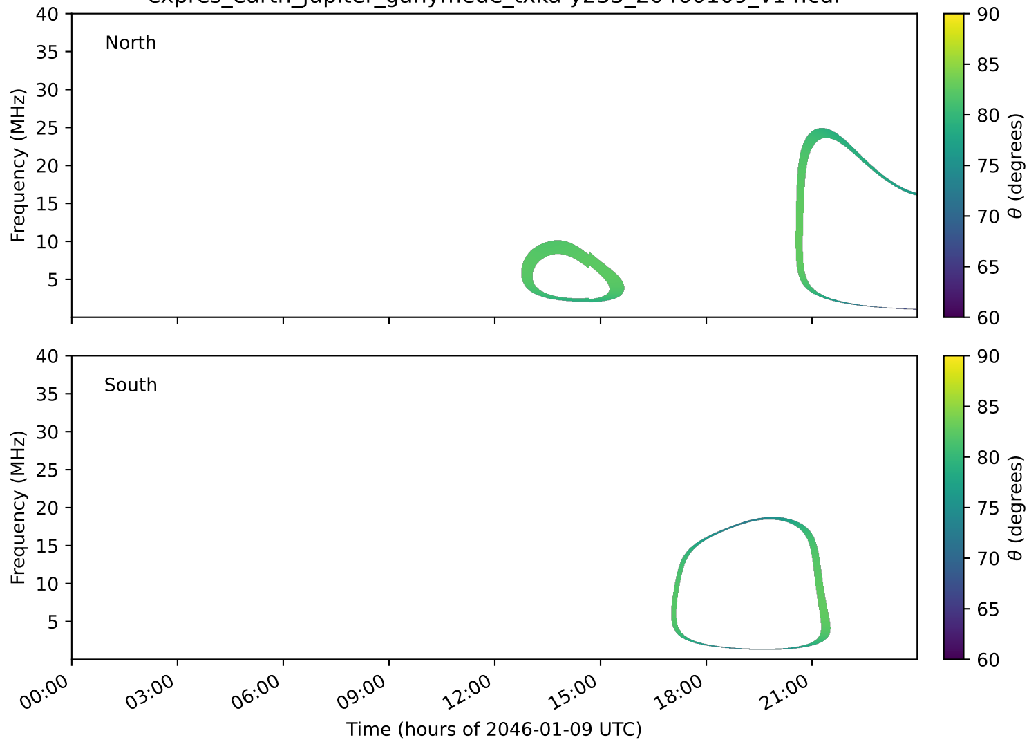
expres_earth_jupiter_ganymede_txka-y235_20460109_v14.cdf
