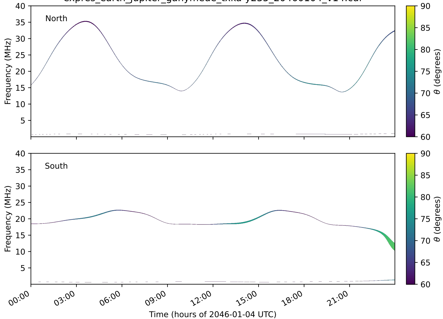
expres_earth_jupiter_ganymede_txka-y235_20460104_v14.cdf
