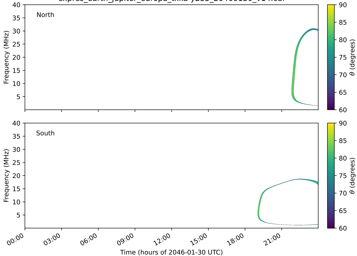
expres_earth_jupiter_europa_txka-y235_20460130_v14.cdf
