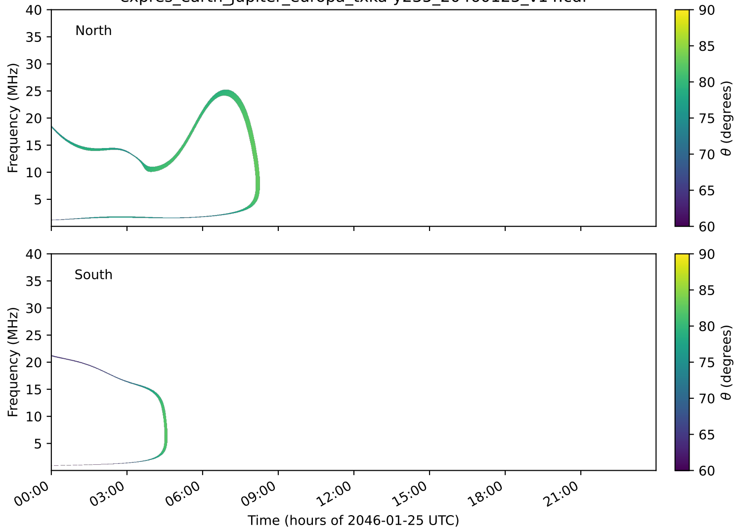
expres_earth_jupiter_europa_txka-y235_20460125_v14.cdf
