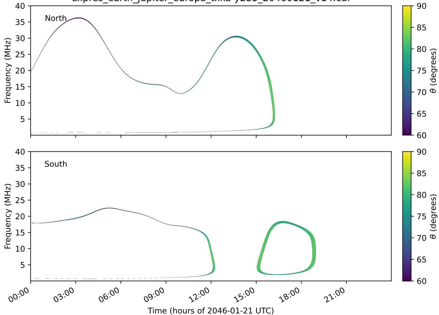
expres_earth_jupiter_europa_txka-y235_20460121_v14.cdf
