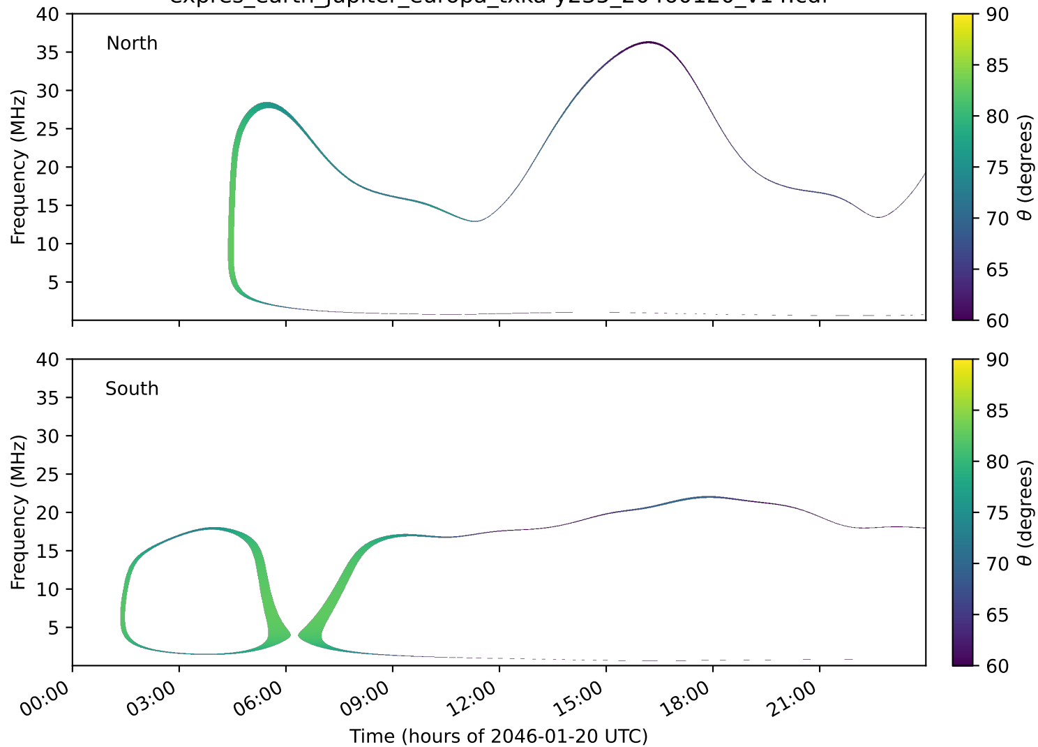
expres_earth_jupiter_europa_txka-y235_20460120_v14.cdf
