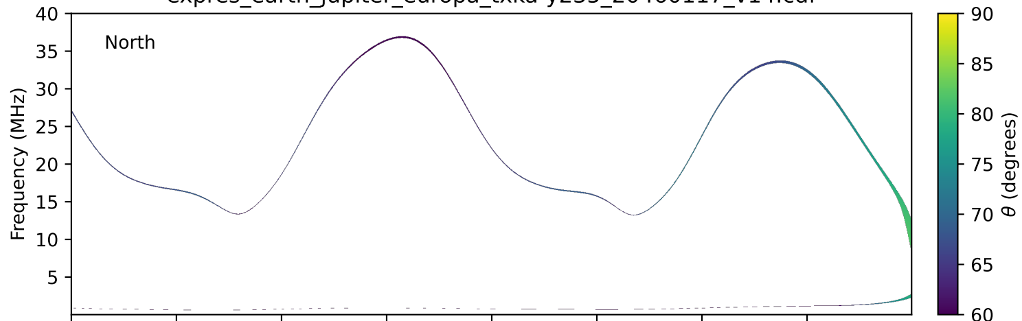
expres_earth_jupiter_europa_txka-y235_20460117_v14.cdf
