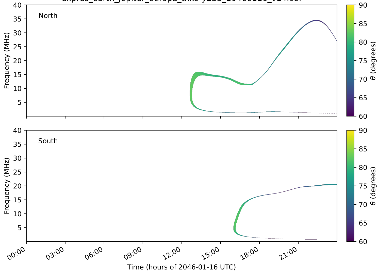
expres_earth_jupiter_europa_txka-y235_20460116_v14.cdf
