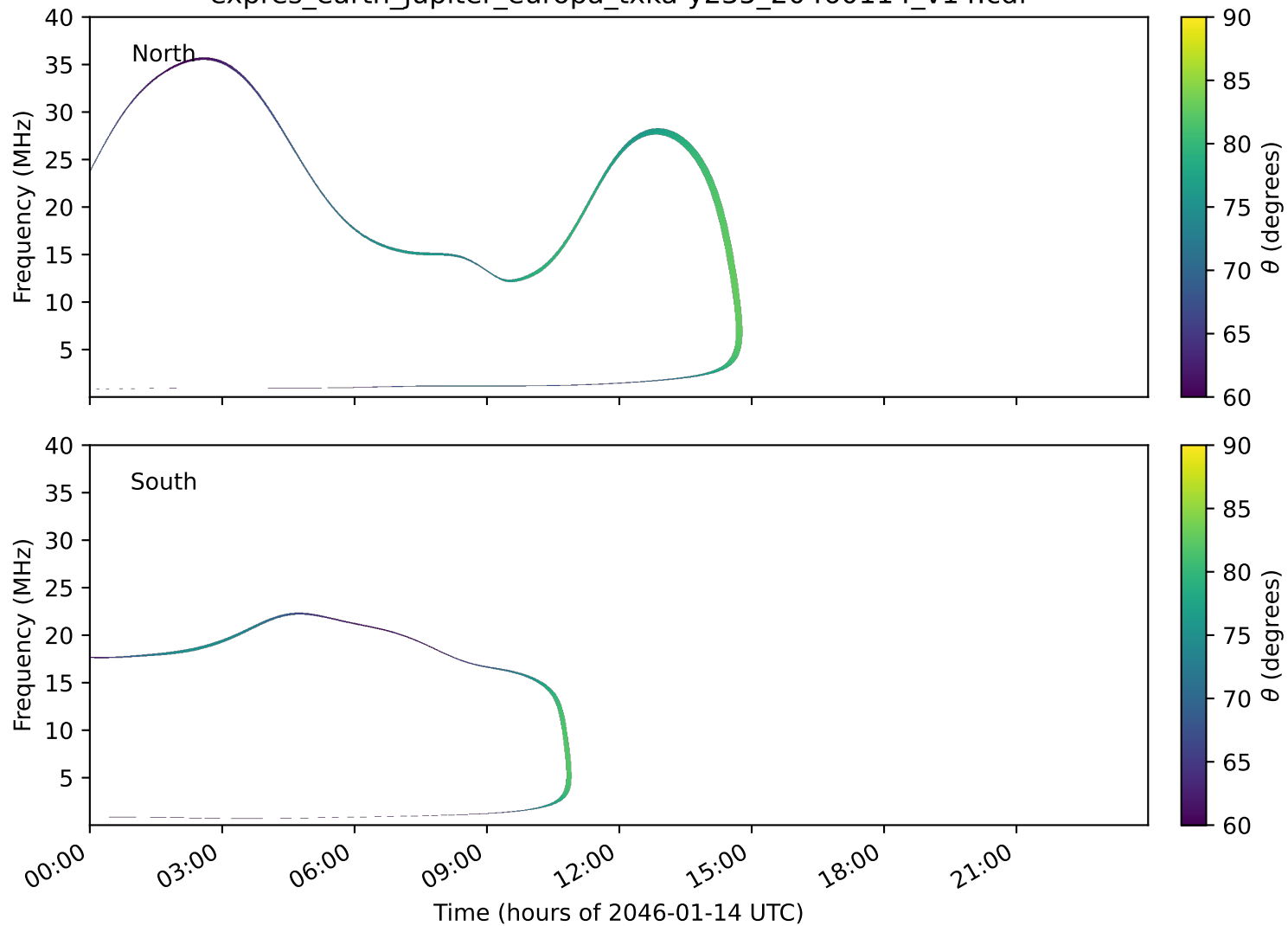
expres_earth_jupiter_europa_txka-y235_20460114_v14.cdf
