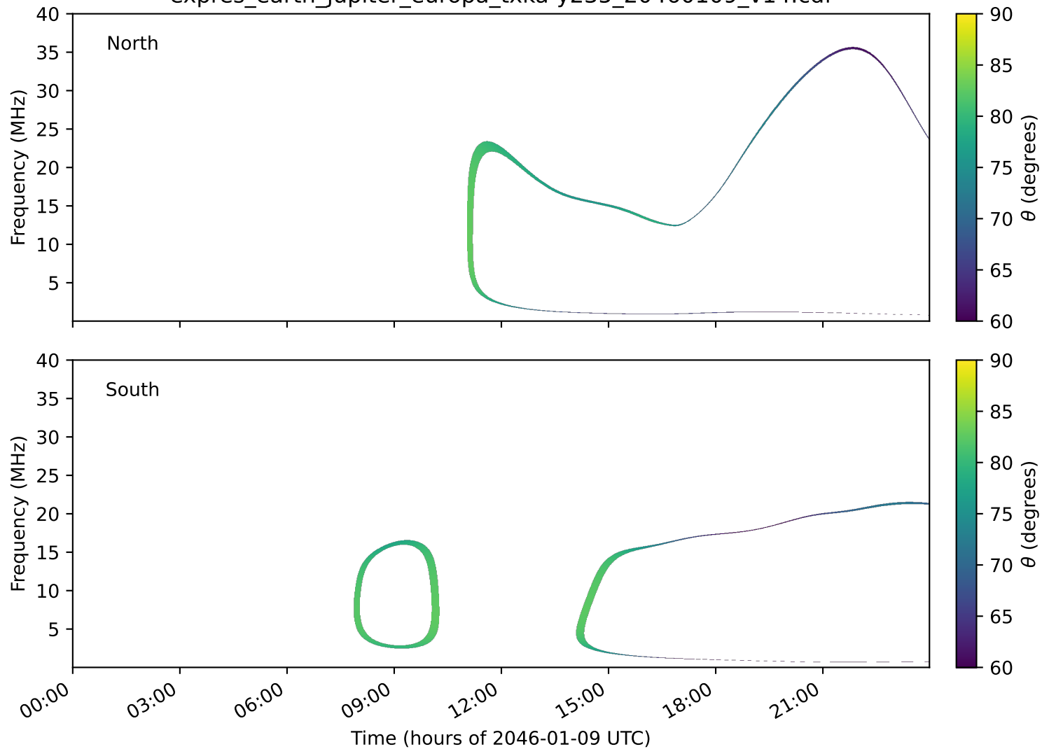
expres_earth_jupiter_europa_txka-y235_20460109_v14.cdf
