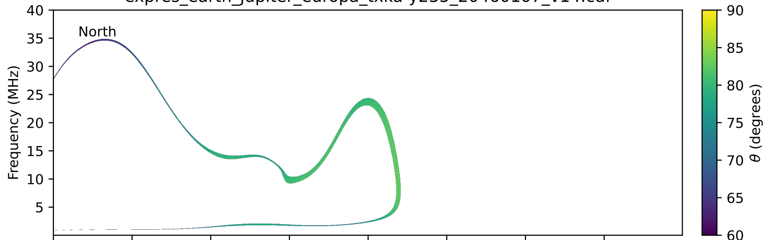
expres_earth_jupiter_europa_txka-y235_20460107_v14.cdf
