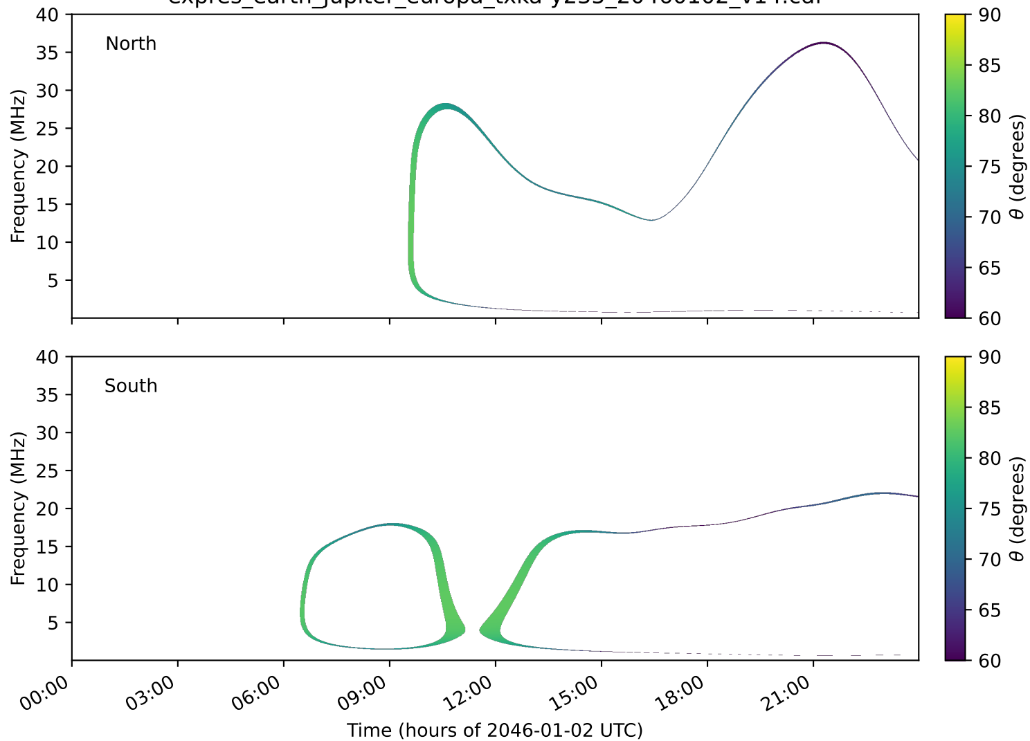
expres_earth_jupiter_europa_txka-y235_20460102_v14.cdf
