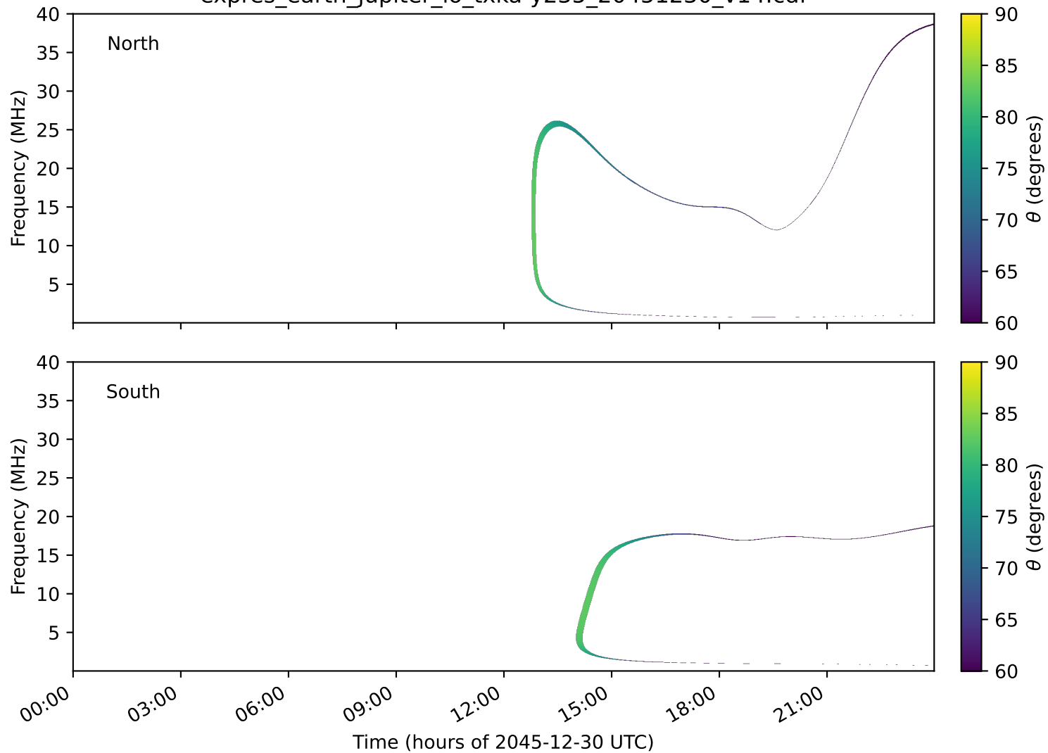
expres_earth_jupiter_io_txka-y235_20451230_v14.cdf
