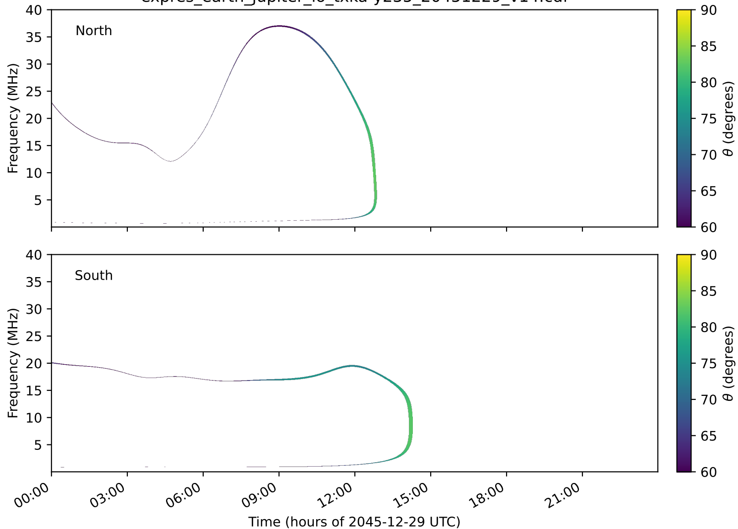
expres_earth_jupiter_io_txka-y235_20451229_v14.cdf
