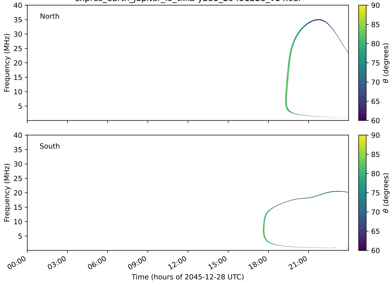
expres_earth_jupiter_io_txka-y235_20451228_v14.cdf
