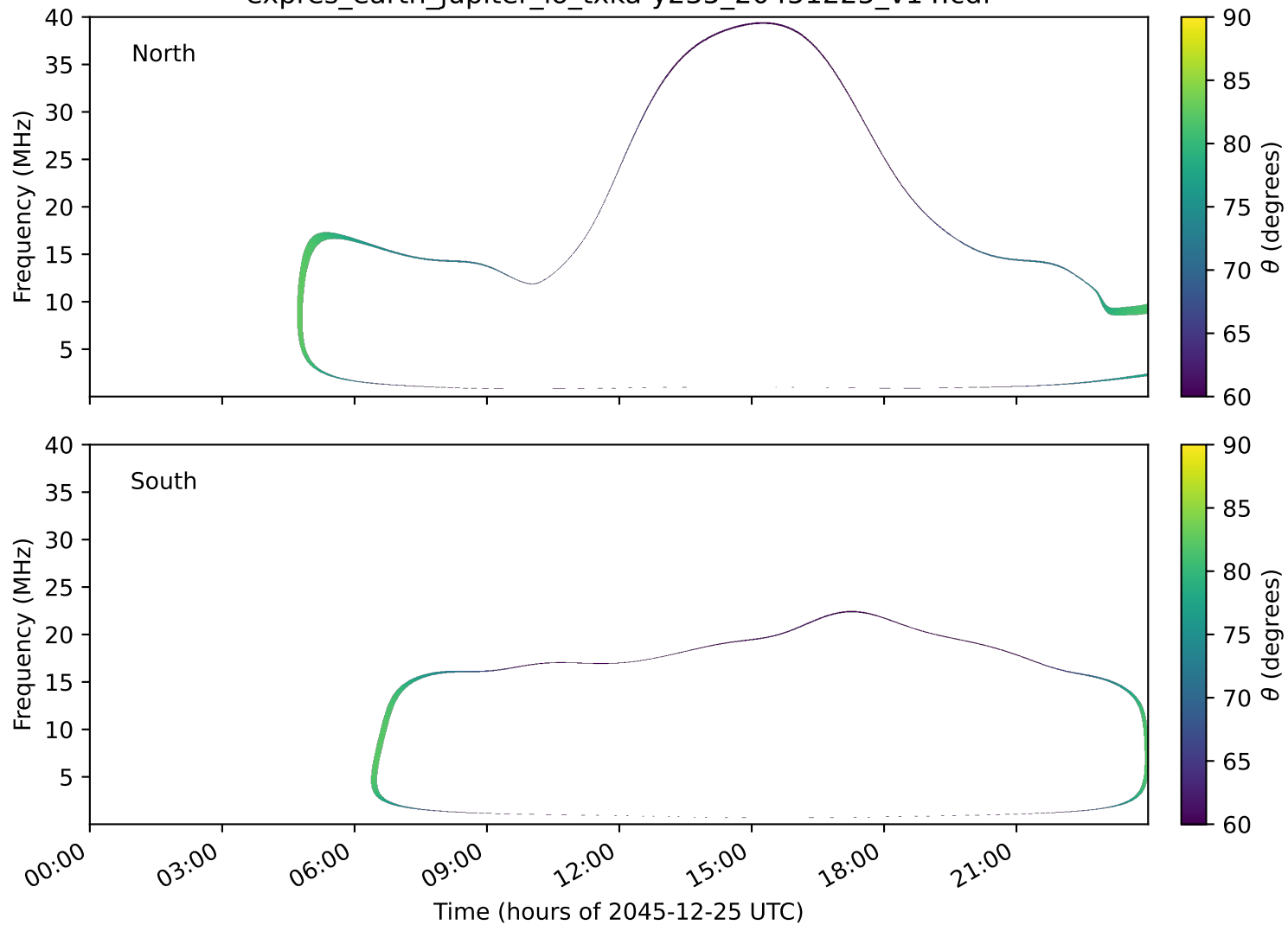
expres_earth_jupiter_io_txka-y235_20451225_v14.cdf
