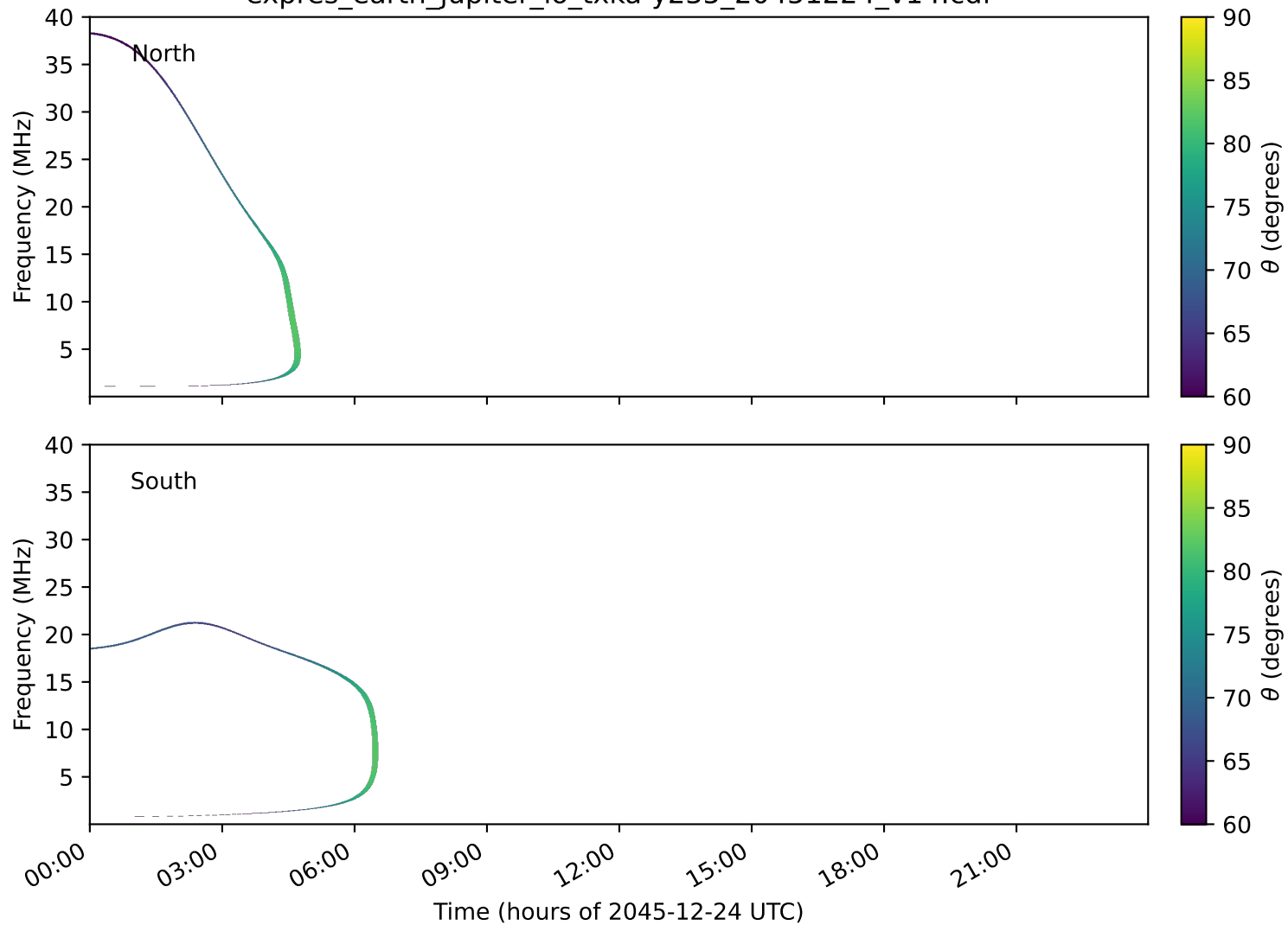
expres_earth_jupiter_io_txka-y235_20451224_v14.cdf
