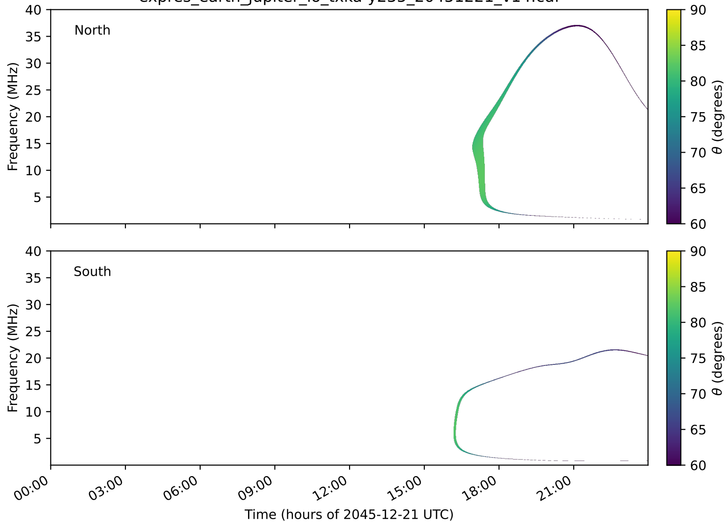
expres_earth_jupiter_io_txka-y235_20451221_v14.cdf
