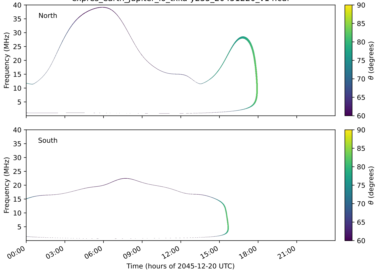
expres_earth_jupiter_io_txka-y235_20451220_v14.cdf
