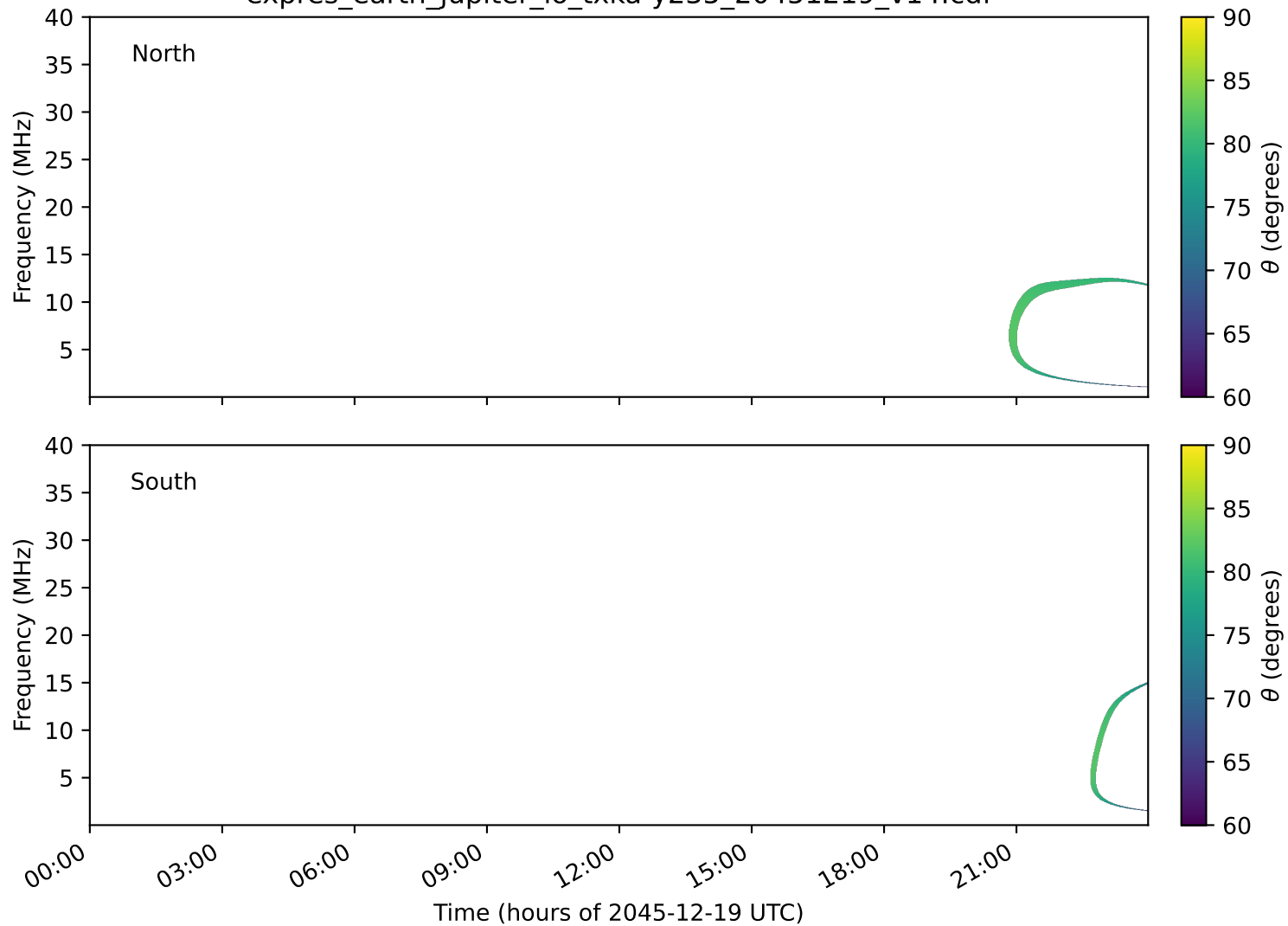
expres_earth_jupiter_io_txka-y235_20451219_v14.cdf
