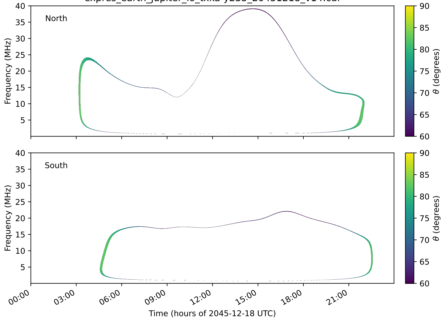
expres_earth_jupiter_io_txka-y235_20451218_v14.cdf
