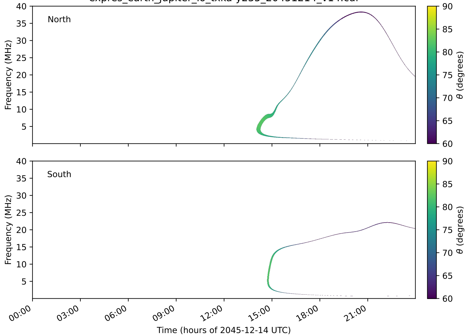
expres_earth_jupiter_io_txka-y235_20451214_v14.cdf
