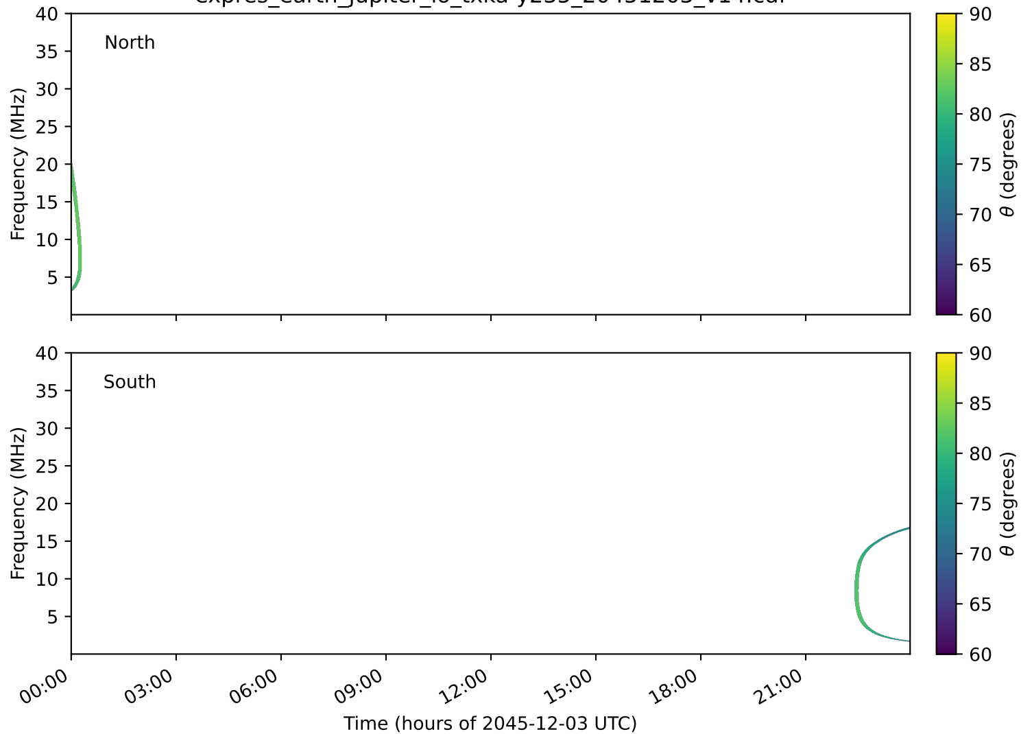
expres_earth_jupiter_io_txka-y235_20451203_v14.cdf
