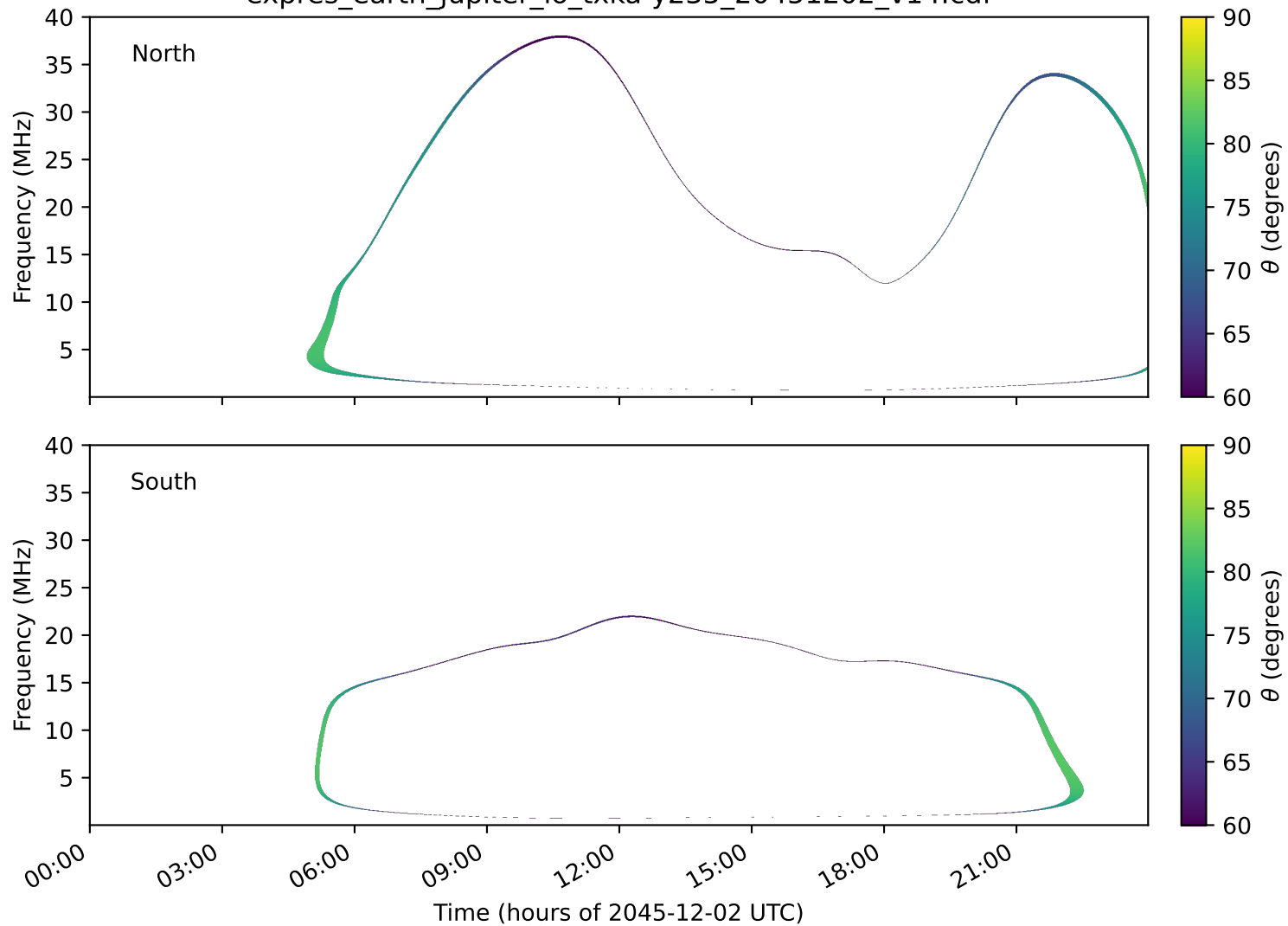
expres_earth_jupiter_io_txka-y235_20451202_v14.cdf
