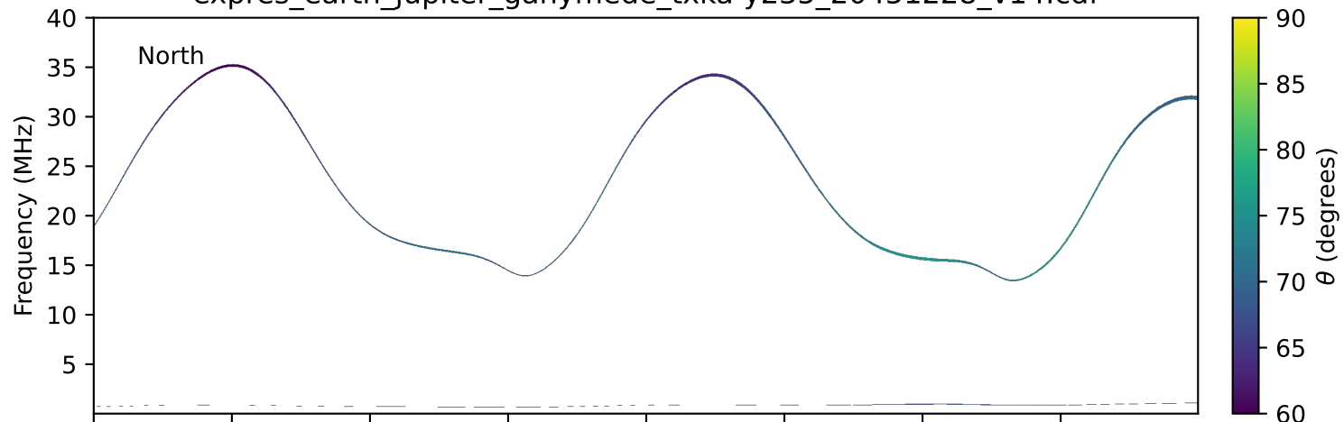
expres_earth_jupiter_ganymede_txka-y235_20451228_v14.cdf
