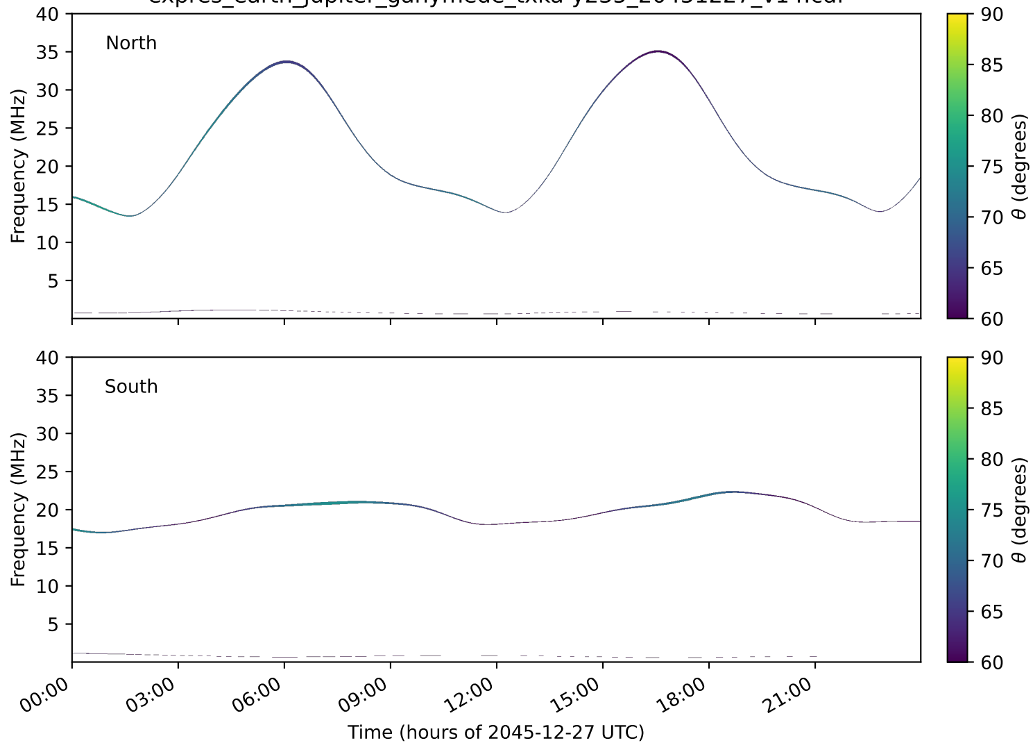
expres_earth_jupiter_ganymede_txka-y235_20451227_v14.cdf
