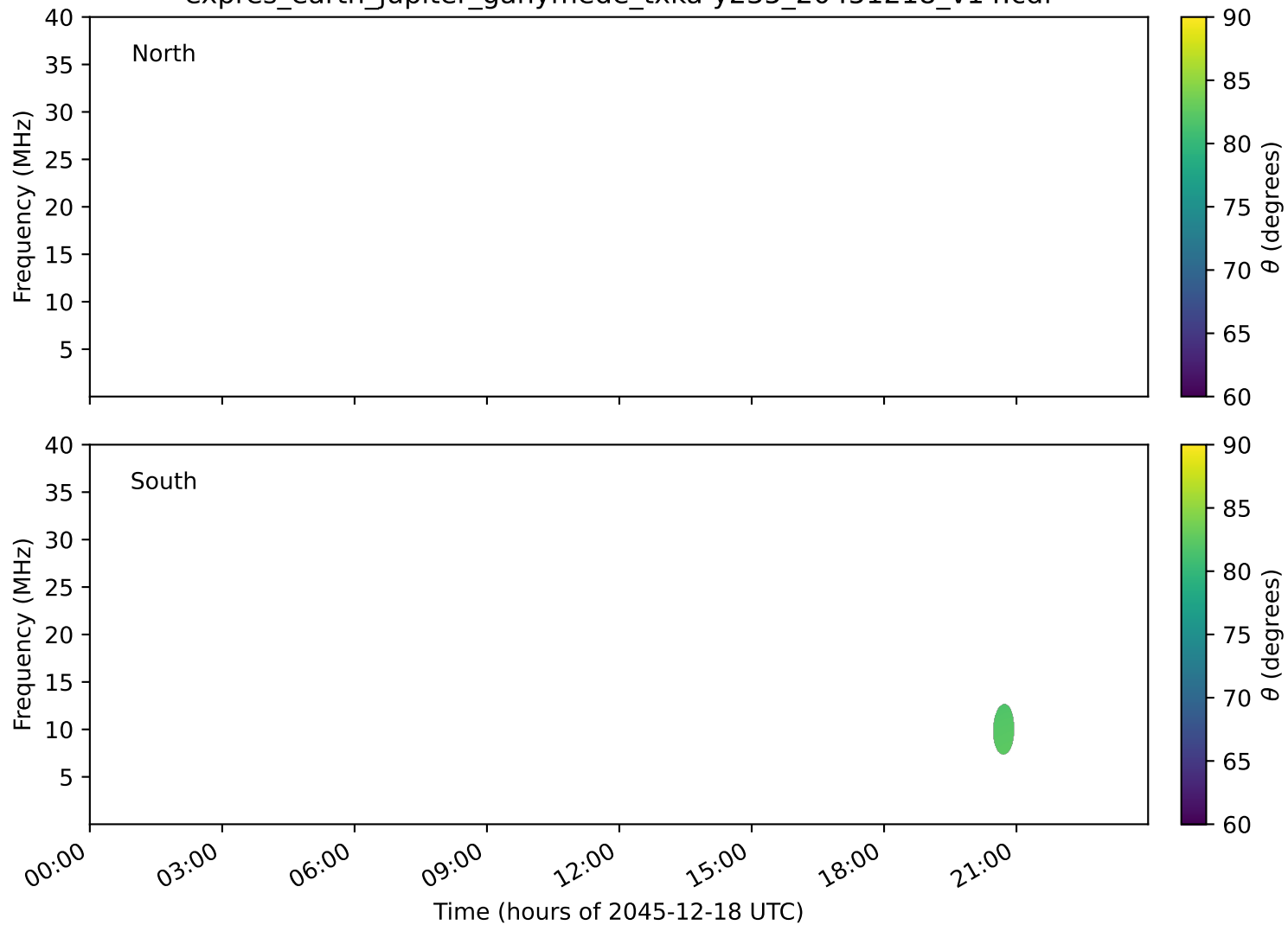
expres_earth_jupiter_ganymede_txka-y235_20451218_v14.cdf
