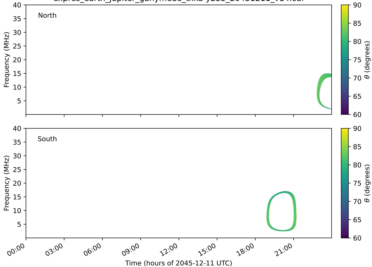
expres_earth_jupiter_ganymede_txka-y235_20451211_v14.cdf
