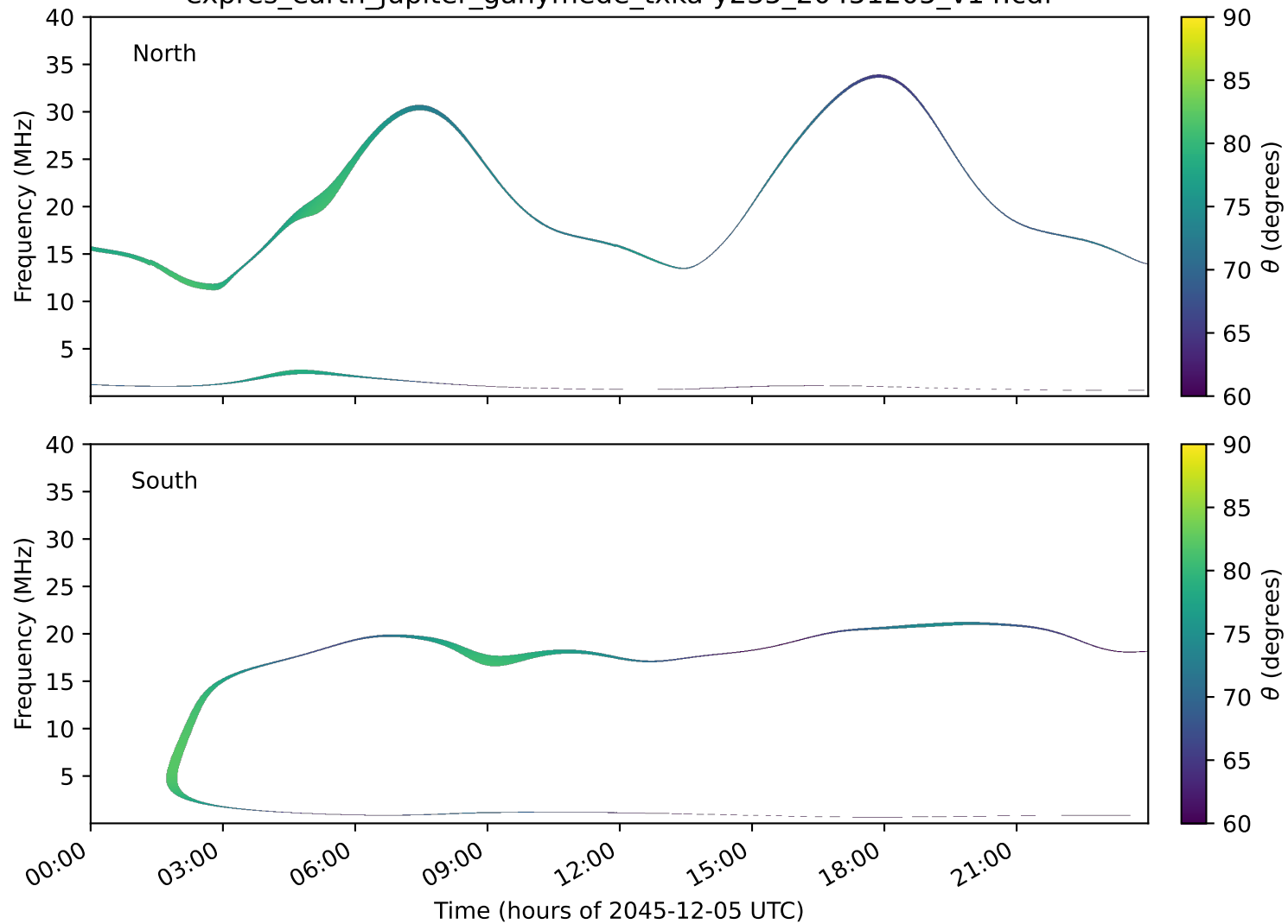
expres_earth_jupiter_ganymede_txka-y235_20451205_v14.cdf
